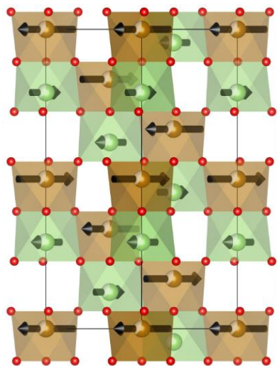
Corundum \text{ScFeO}_3/\text{GaFeO}_3
